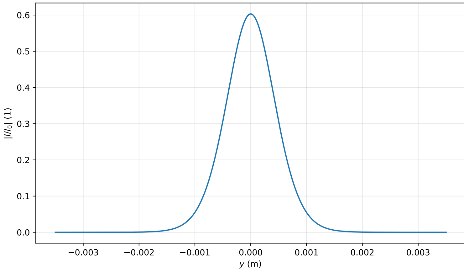
Intensity profile I(x=0, y, z=2.468)/I_0 , P_{in}=0.4P_{cr} , artificial time
